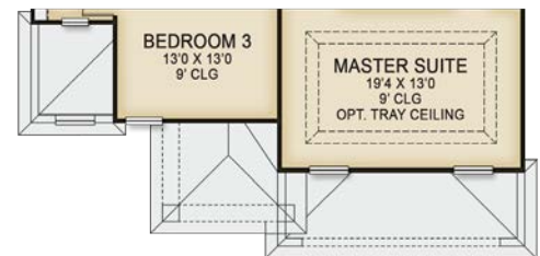
SECOND FLOOR C
